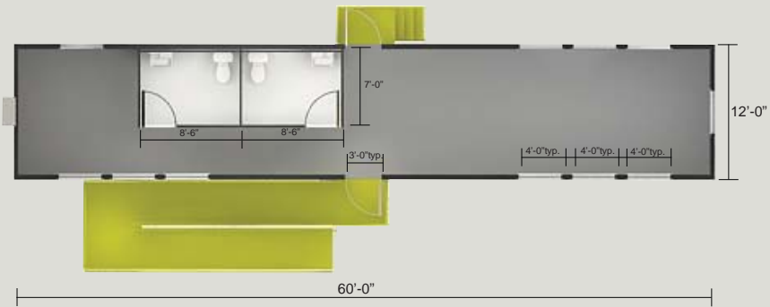
Floor plan
