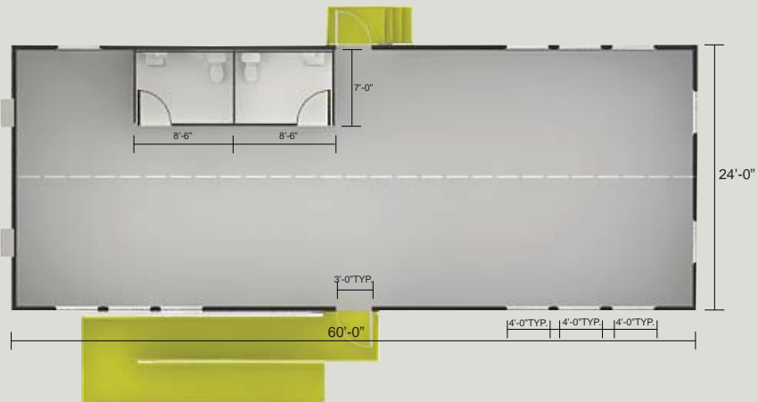
Floor plan
