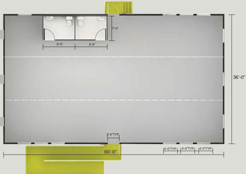
Floor plan
